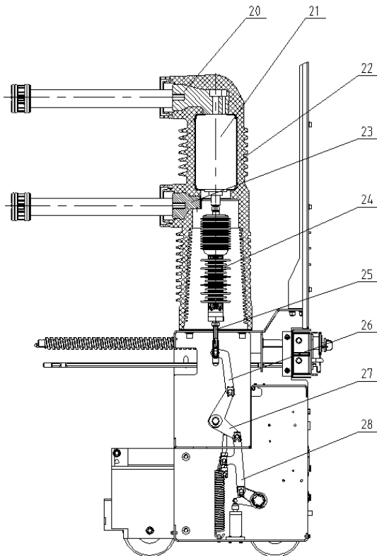
Fig. 3 internal structure diagram of circuit breaker (floor type)
